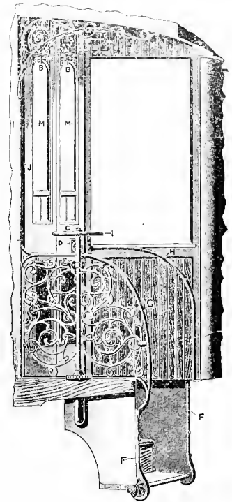
Fig. 3772. Sectional View. VESTIBULED PLATFORM, AND ITS TRIMMINGS.
